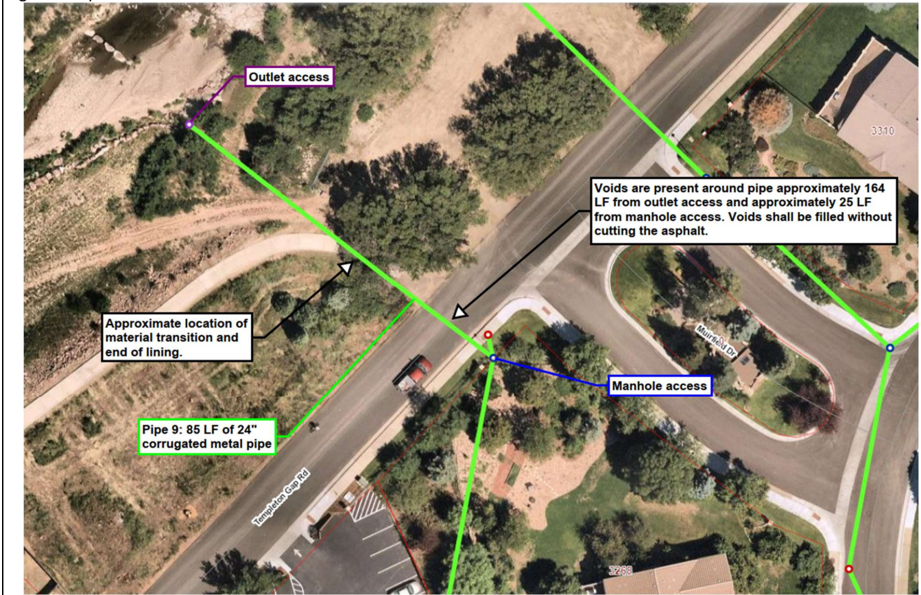
Figure 8: Pipe 9 to be lined on Templeton Gap Rd
