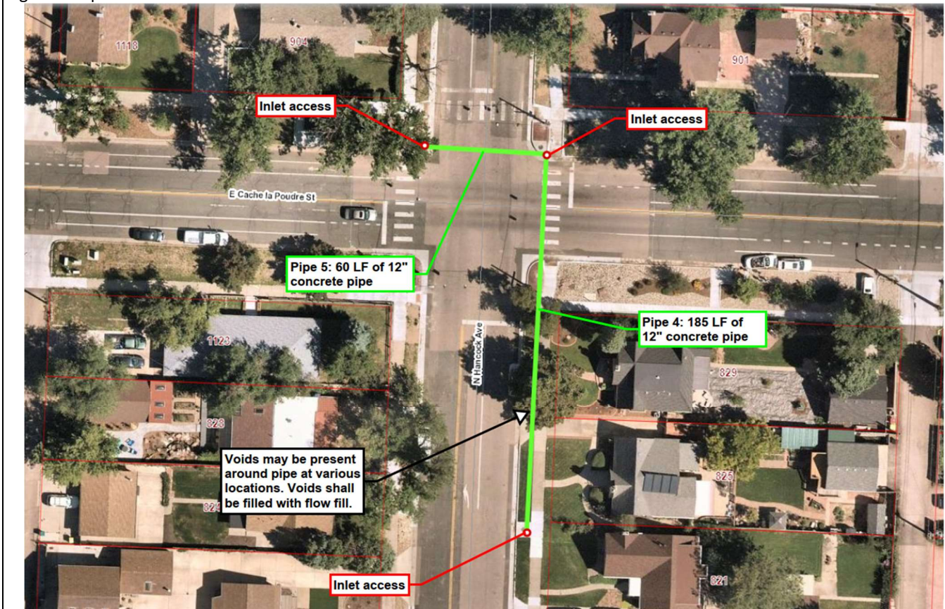
Figure 4: Pipe 4 and Pipe 5 to be lined on N Hancock Ave
