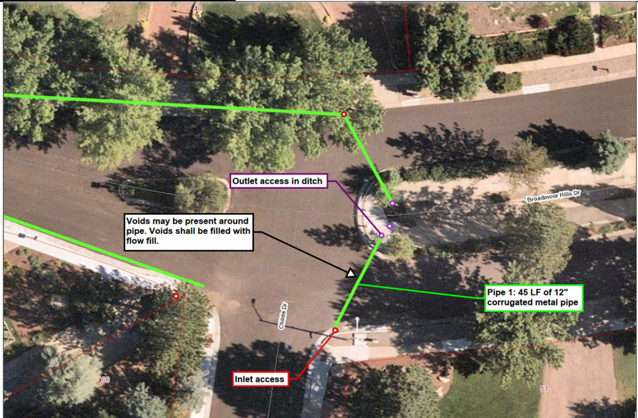
Figure 1: Pipe 1 to be lined on Broadmoor Hills Dr
