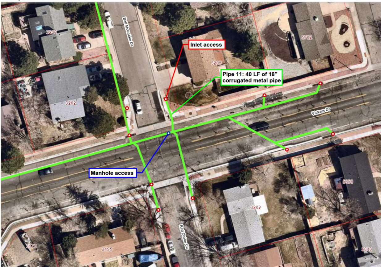
Figure 10: Pipe 11 to be lined on Vickers Dr
