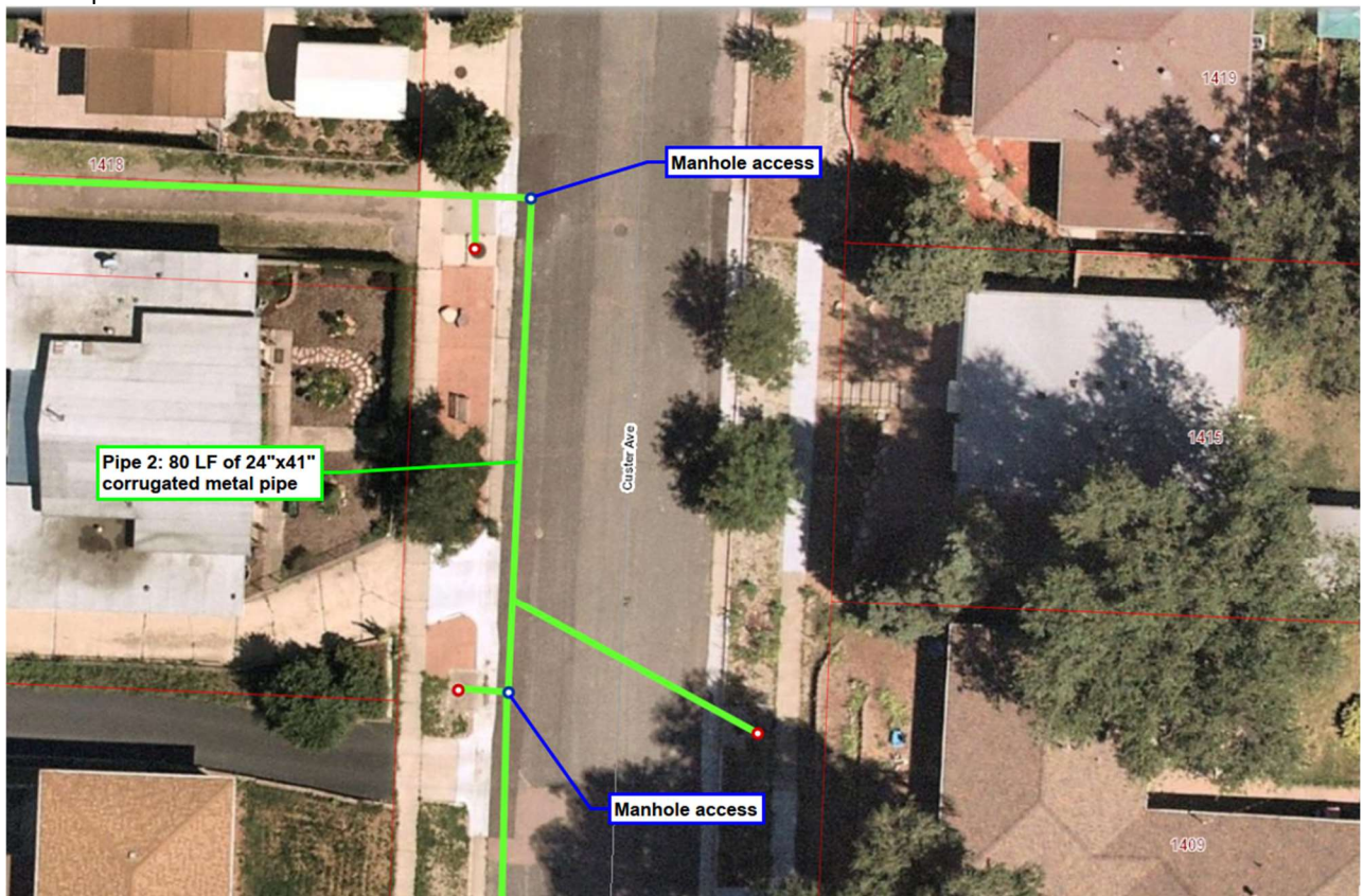
Figure 2: Pipe 2 to be lined on Custer Ave
