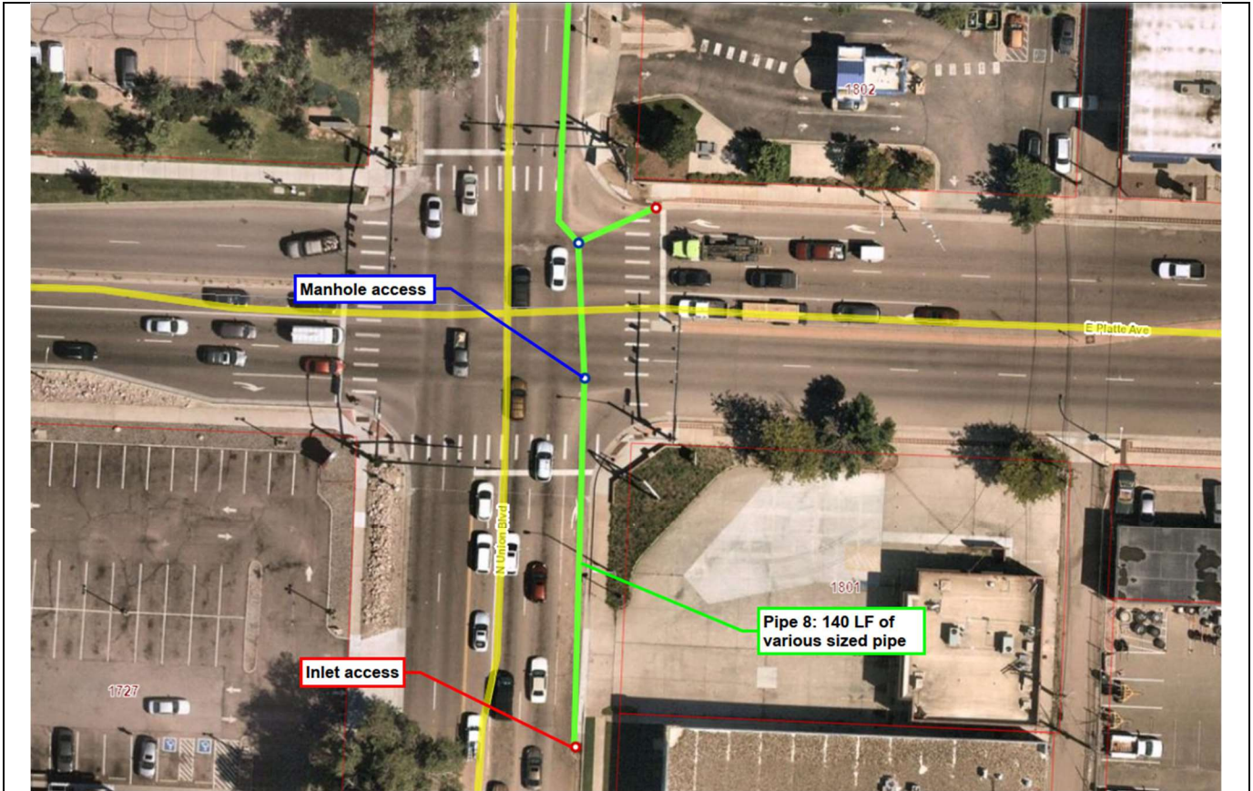
Figure 7: Pipe 8 to be lined on Platte Ave
