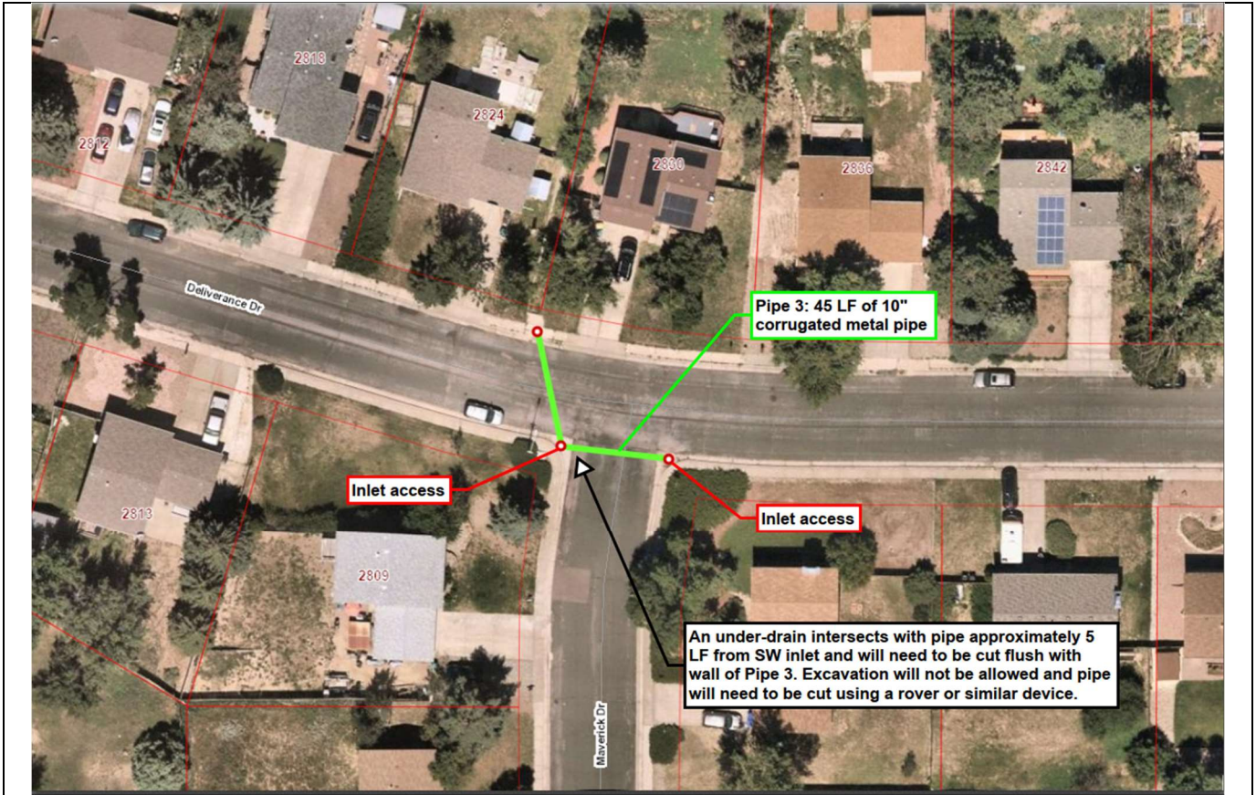
Figure 3: Pipe 3 to be lined on Deliverance Dr
