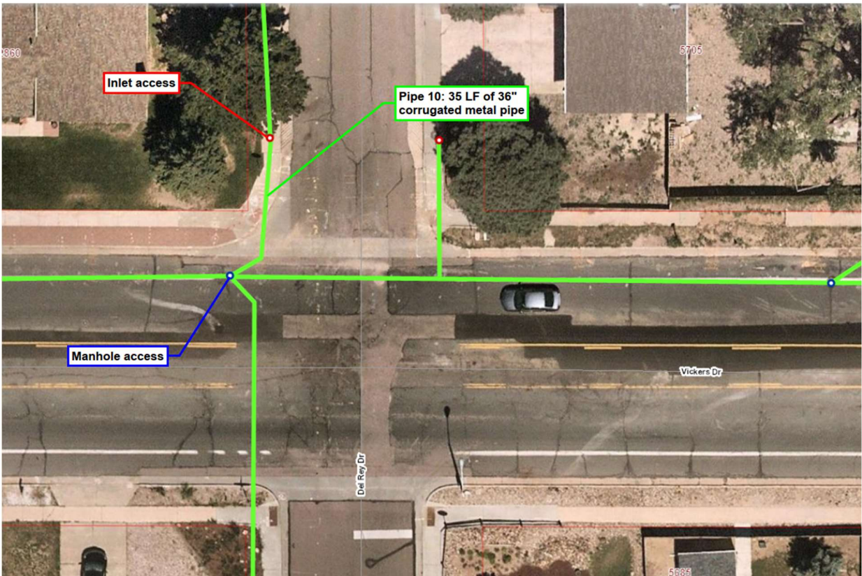
Figure 9: Pipe 10 to be lined on Vickers Dr
