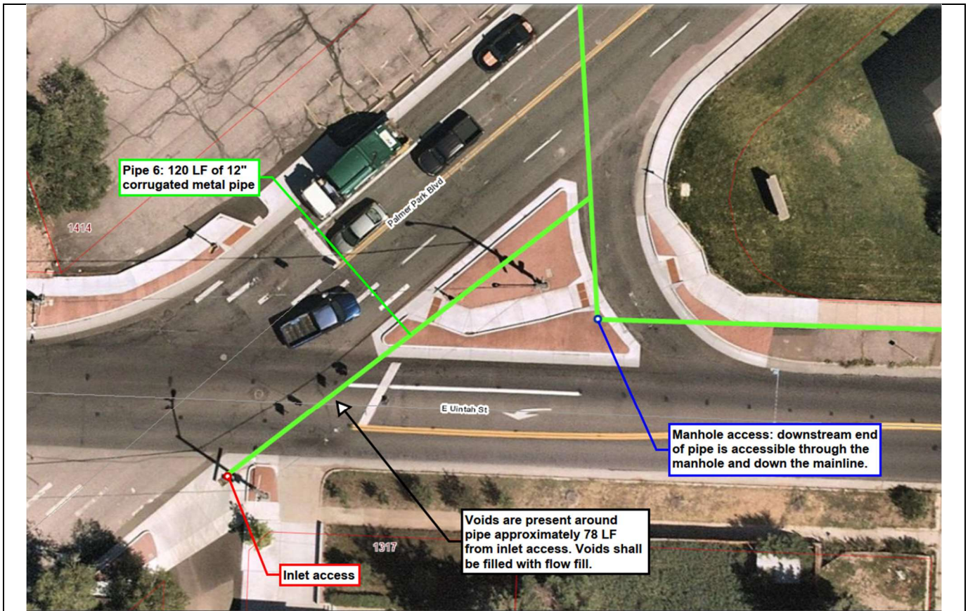
Figure 5: Pipe 6 to be lined on Palmer Park Blvd
