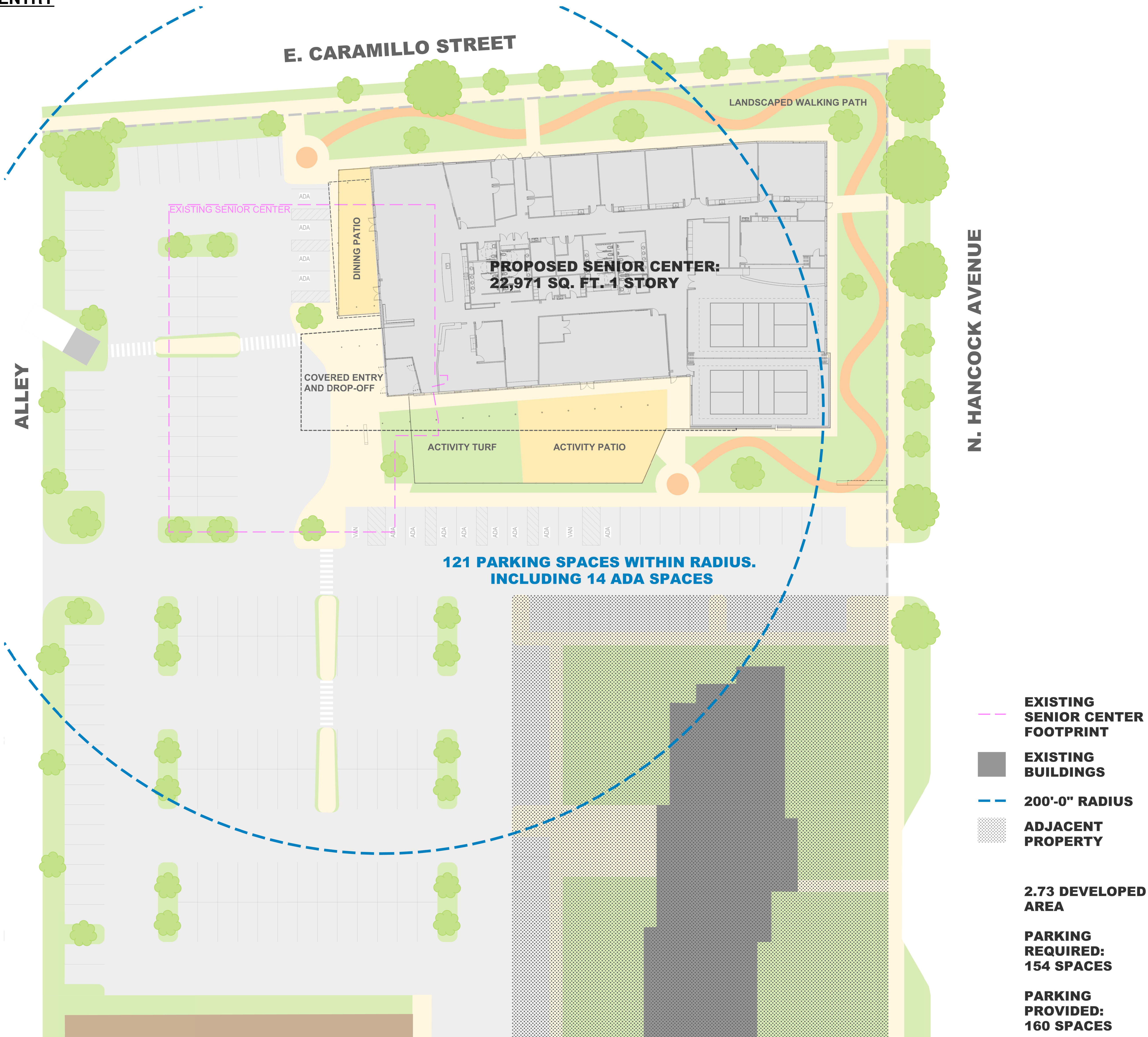
PROPOSED SITE PLAN
